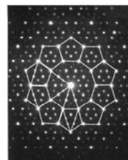
Analysis of quasi-crystal diffraction diagram. R Henry 2007
