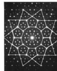
Analysis of quasi-crystal diffraction diagram. R Henry 2007
